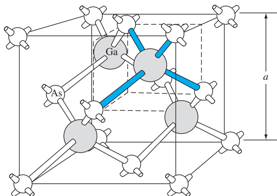
Figure 1.14 | The zincblende (sphalerite) lattice of GaAs.
