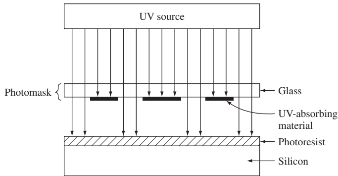
Figure 0.2 | Schematic showing the use of a photomask.
