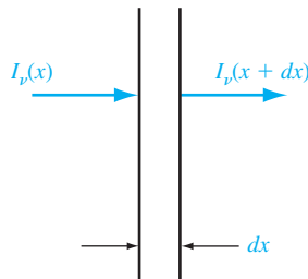
Figure 14.2 | Optical absorption in a differential length.
