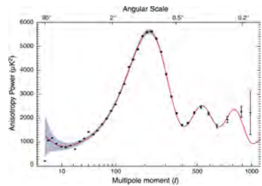
Figure 19.2: Power spectrum corresponding to the data shown in Fig. 19.1 (see Eq. 19.3.) The continuous line shows the best fit of a model that assumes Dark Matter to be cold (see text). [From WMAP collaboration. (6) ]
