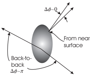
Figure 16.10: Sketch of two-particle emission from fireball.
