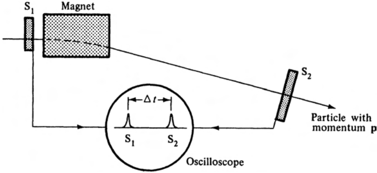
Figure 5.8: Determination of the mass of a particle by selecting its momentum p and measuring its velocity v .
