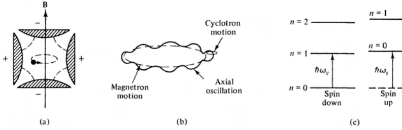
Figure 6.8: (a) Penning trap—a combination of a magnetic field B and a cylindrical electric quadrupole field. (b) Motion of an electron in the combined fields of the Penning trap. (c) Magnetic energy levels of the electron in the trap.
