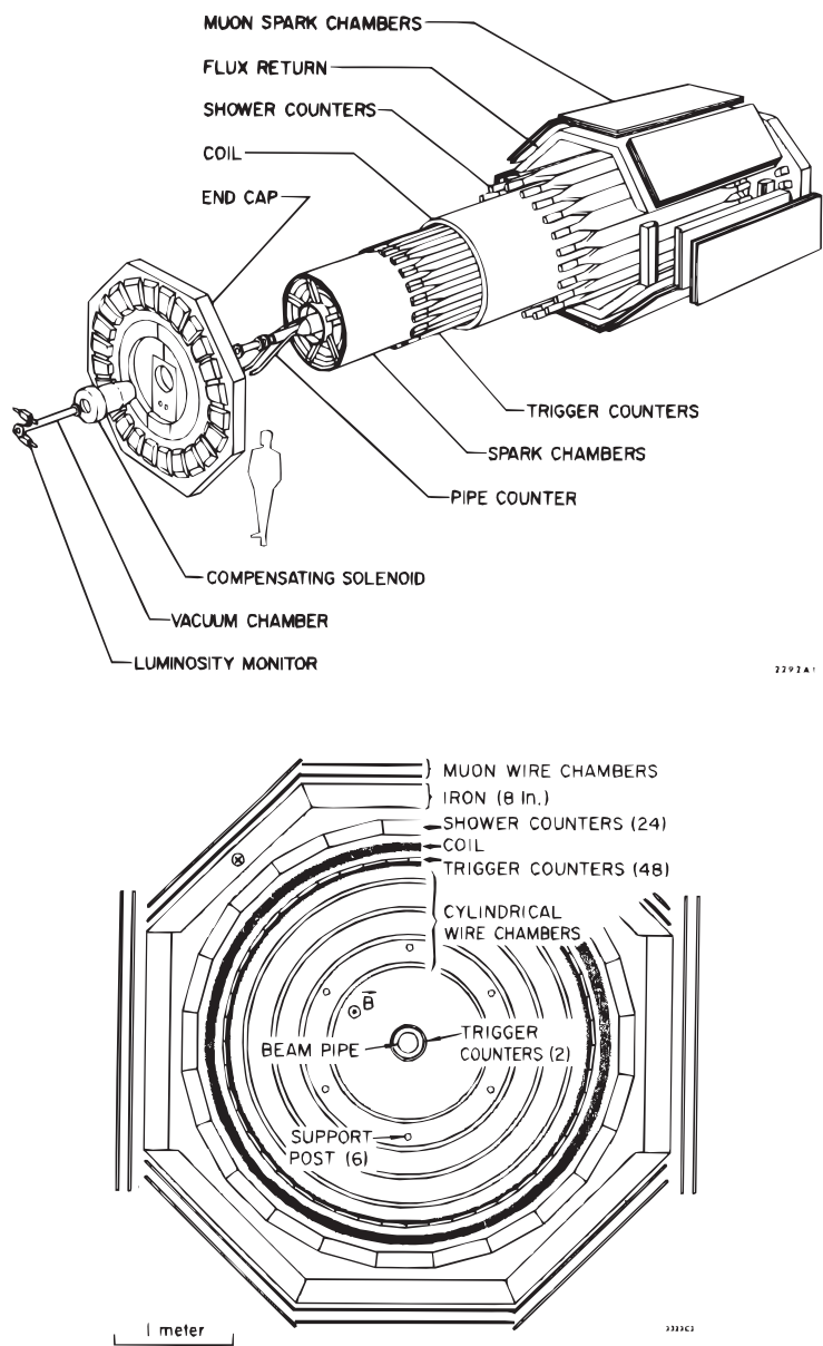
Figure 10.20: Magnetic detector at SPEAR. The detector included spark chambers, scintillation counters, and a solenoid. The solenoid was 3 m in diameter, 3 m long, and produced a 4 kG field parallel to the beam. [Figure courtesy of SLAC.]
