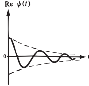
Figure 5.16: Real part of the wave function of a decaying state. It is assumed that the decaying state is formed at t = 0 .
