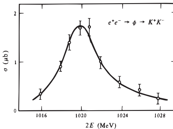
Figure 10.16: Cross section for the process e^+e^- \rightarrow K^+K^- . [From V. A. Sidorov (NOVOSIBIRSK), Proceedings of the 4th International Symposium on Electron and Photon Interactions , (D. W. Braben, ed.), Daresbury Nuclear Phys. Lab, 1969.]
