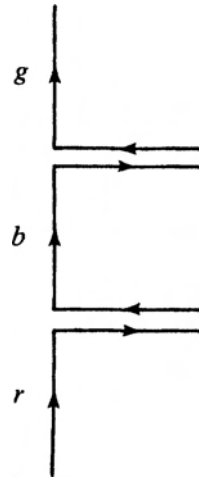
Figure 14.22: The emission of two gluons by a red quark.
