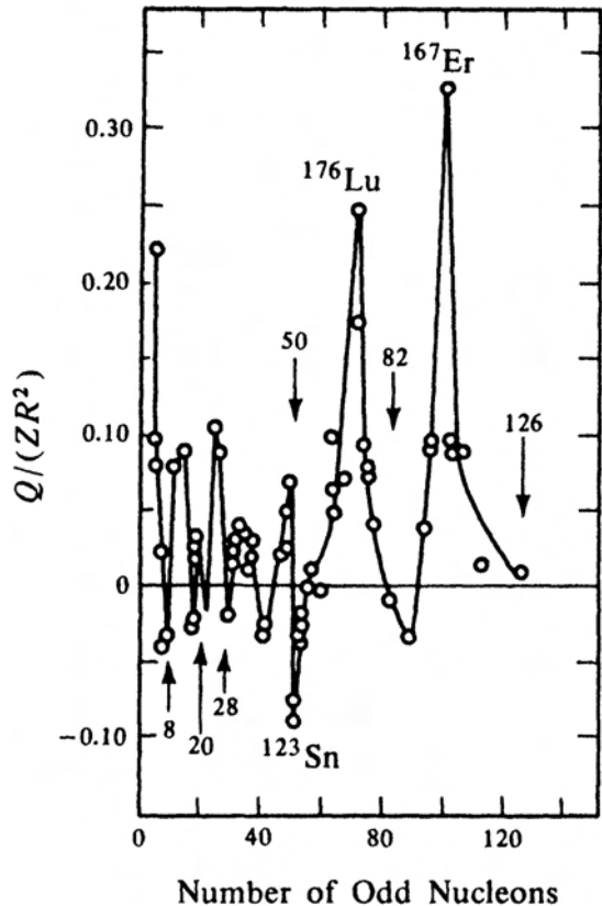
Figure 18.1: Reduced quadrupole moment plotted versus the number of odd nucleons ( A or N ). Arrows indicate the positions of closed shells, where \mathcal{Q} = 0 .
