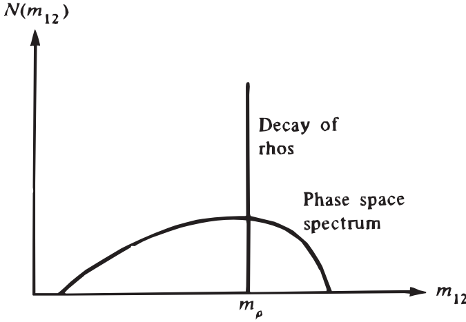
Figure 5.11: Invariant mass spectrum if pion pairs are produced independently (phase space) or if they result from the decay of a rho of small decay width.
