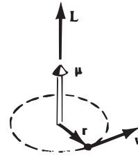
Figure 5.4: A particle of mass m and charge q on a circular orbit produces a magnetic moment \mu and an orbital angular momentum \mathbf{L} .
