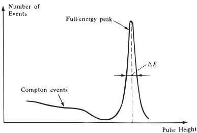
Figure 4.3: Scintillation spectrum, NaI(Tl) crystal.
