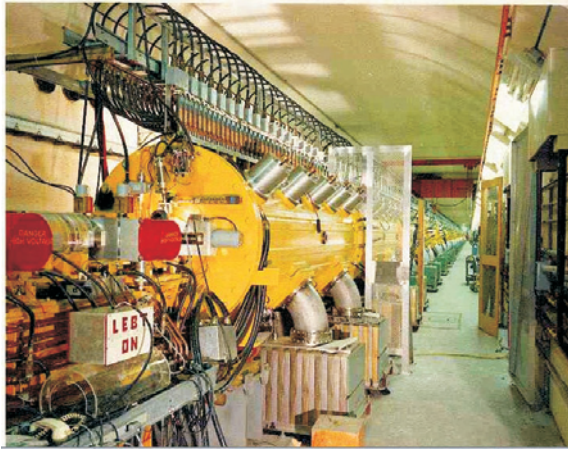
Photo 2: A view of the linac at RHIC. Its purpose is to provide currents of up to 35 milliamperes of protons at energies \approx 200 MeV for injection in a synchrotron for further acceleration. The basic components of the linac include a radiofrequency quadrupole pre-injector, and nine accelerator radiofrequency cavities spanning the length of a 150 meters tunnel (shown above.) [Courtesy of Brookhaven National Lab.]
