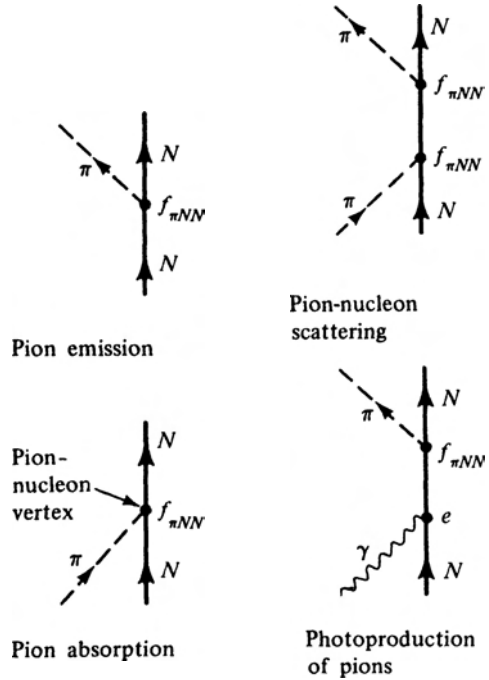
Figure 14.3: Pions can be emitted and absorbed singly. The strength of the pion-nucleon interaction is characterized by the coupling constant f_{\pi NN} .
