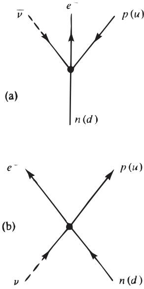
Figure 11.3: Neutron decay and neutrino absorption. It is assumed that the absolute values of the matrix elements for the two processes are the same. The diagrams apply to quarks with u and d substituting for p and n .
