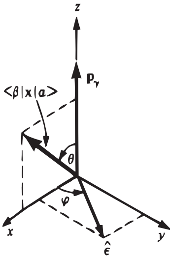
Figure 10.6: The polarization vector \hat{\mathbf{e}} of a photon emitted along the z axis lies in the xy plane. The vector \langle \beta | \mathbf{x} | \alpha \rangle , describing the decaying system, is taken to lie in the xz plane.
