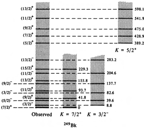
Figure 18.7: Energy levels of ^{249}\text{Bk} . All observed energy levels up to an excitation energy of about 600 keV are given at the left. The levels fall into three rotational bands; these are shown at the right. All energies are in keV.
