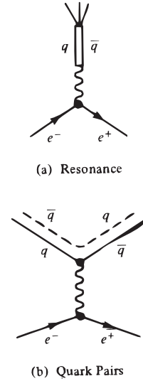
Figure 10.23: Production of (a) resonance and (b) of “individual” quark pair. In (b), the second q\bar{q} pair shown is required to produce observable mesons.
