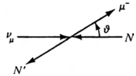
Figure 11.17: "Elastic" reaction \nu_\mu N \rightarrow \mu^- N' in the c.m.
